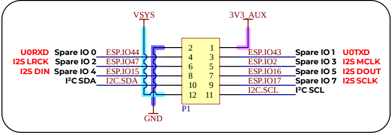
Expansion Connector
