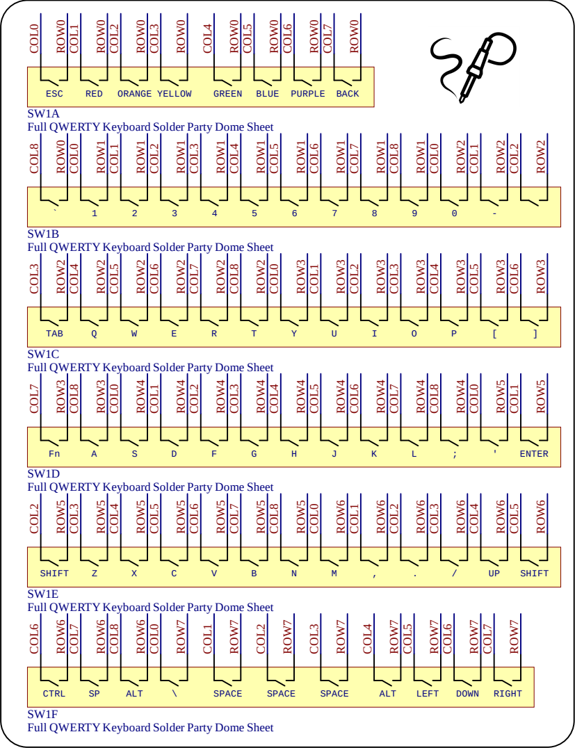
Solder Party KeebDeck
