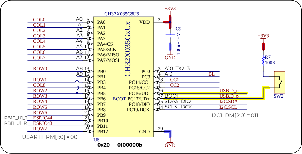
Solder Party KeebDeck
